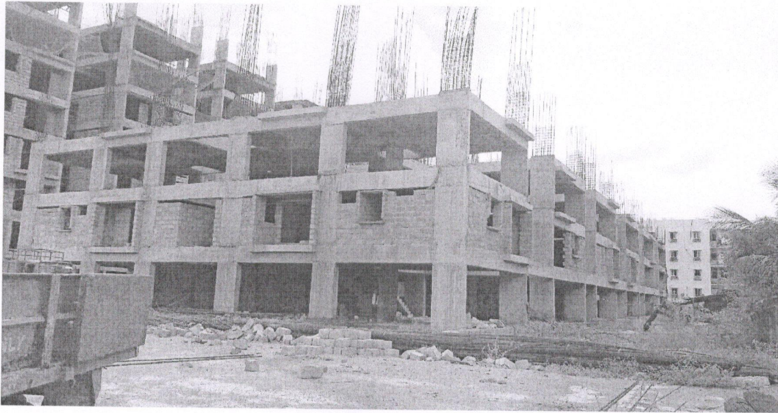
Block C1: Eight Floor Level slab 1 st half concrete casting 100% completed. Shuttering & barbending work on progress for 2 nd half of Eight Floor level slab.
